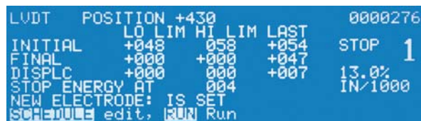
LVDT Screen – Program limits and view results.
